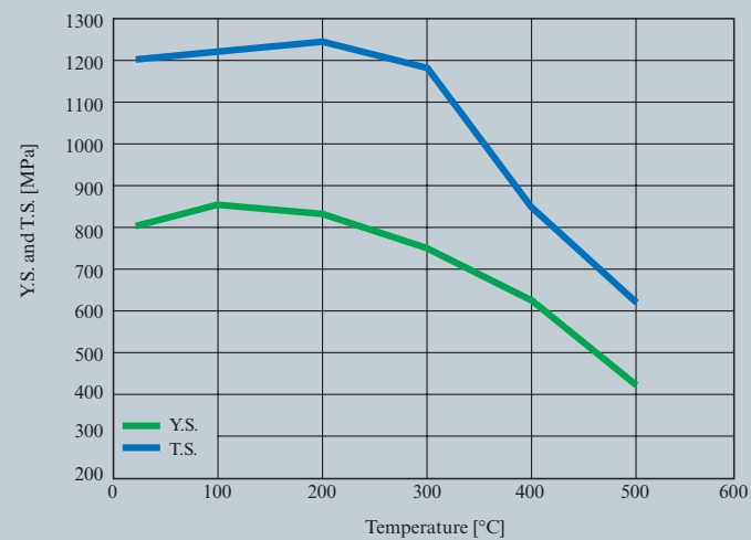
Figure 8: Effect of temperature on the yield and tensile strength of DILLIDUR 400 V (auxiliary data, plate thickness = 20 mm)
