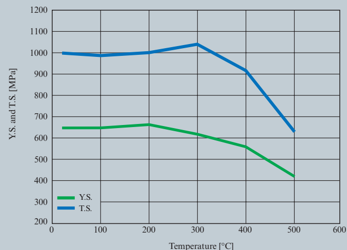
Figure 7: Effect of temperature on the yield and tensile strength of DILLIDUR 325 L (auxiliary data, plate thickness = 20 mm)
